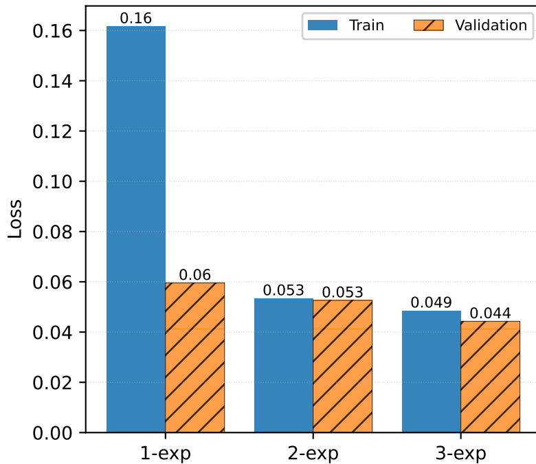
Total Loss
