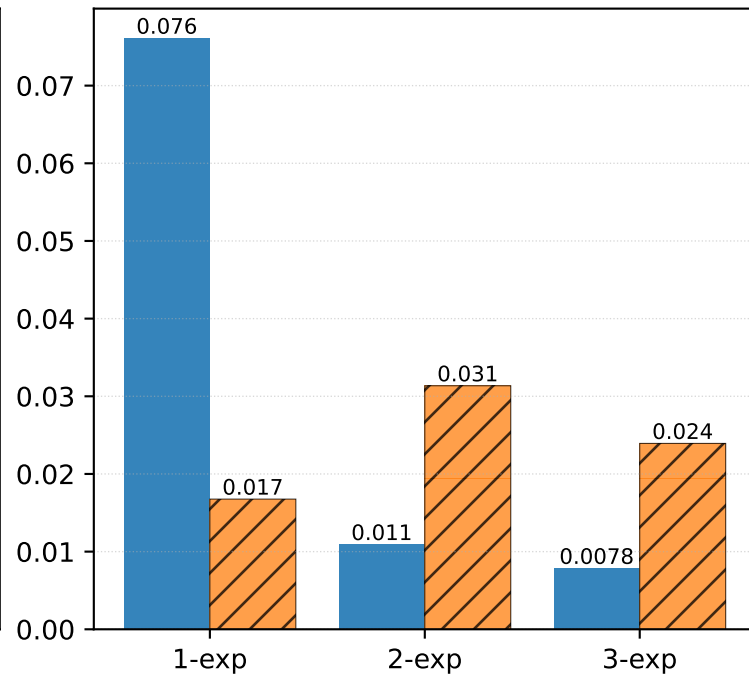
Convolution Loss
