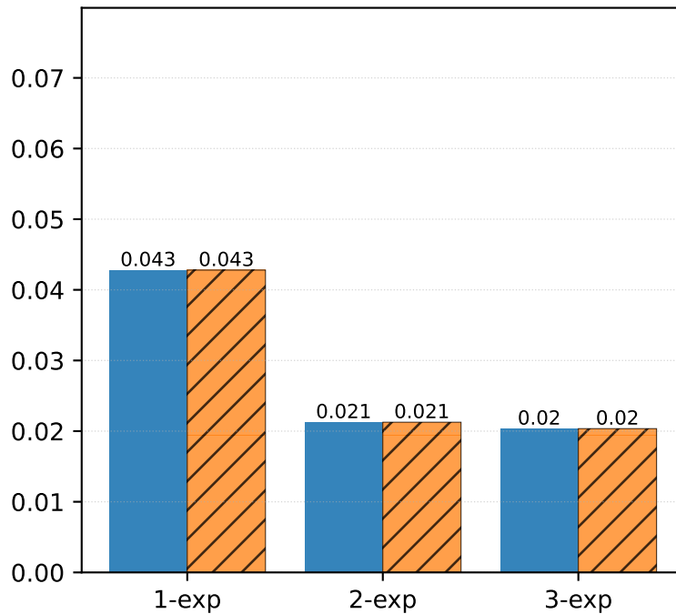
Orbit Loss
