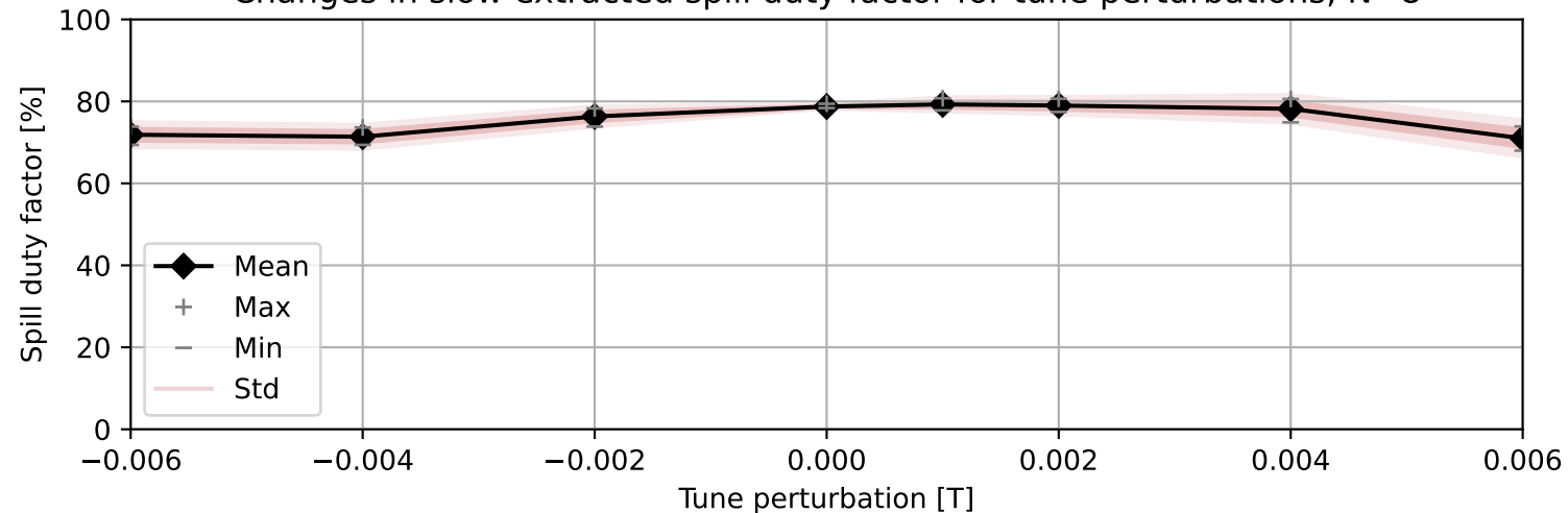
Changes in slow extracted spill duty factor for tune perturbations, N=8
